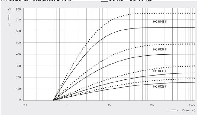
Pumping speed
