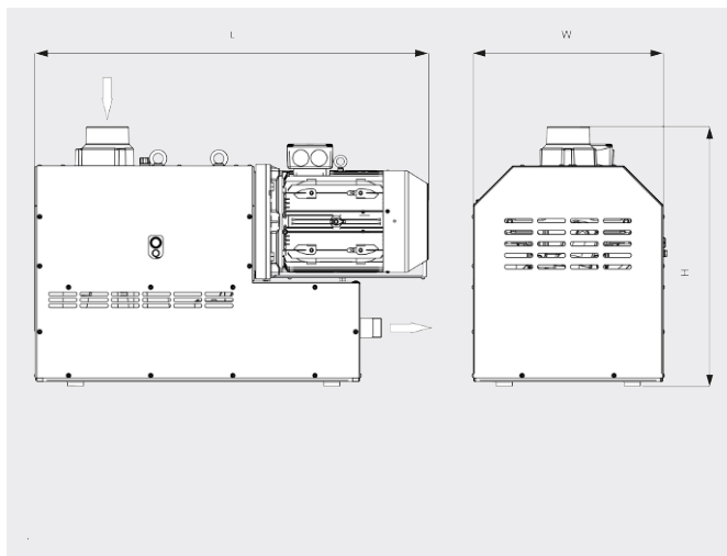
Dimensional drawing
