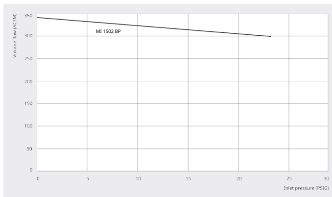
Volume flow
