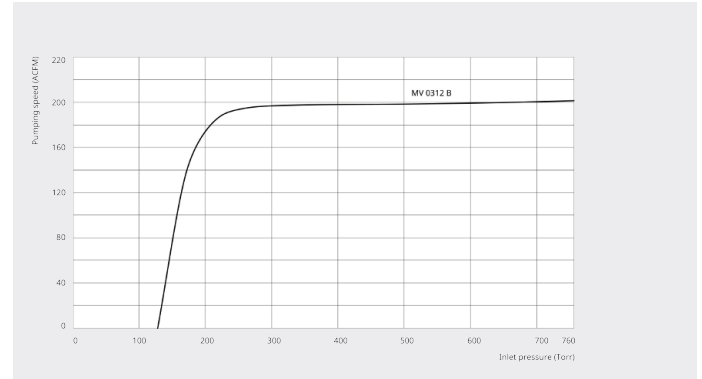
Pumping speed
