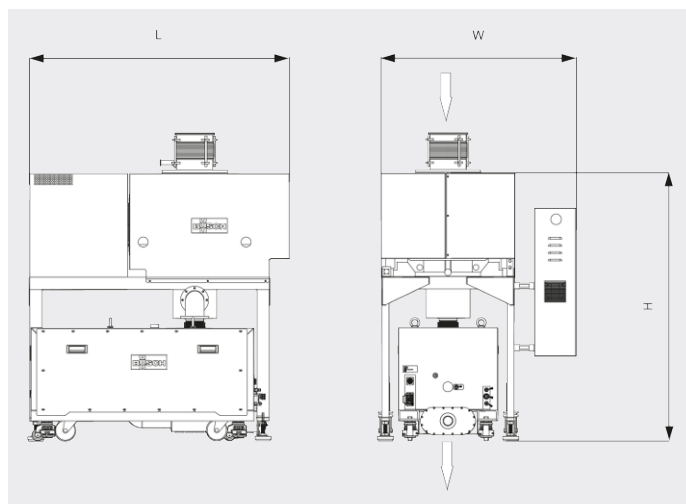
Dimensional drawing
