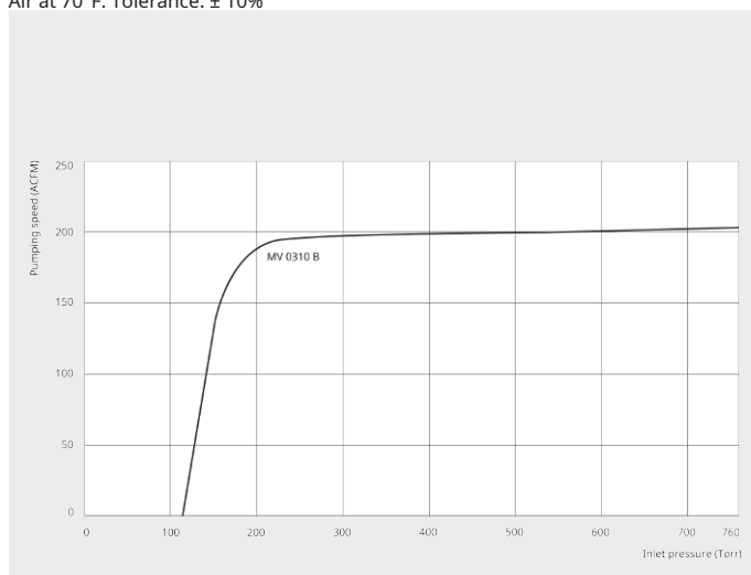
Pumping speed
