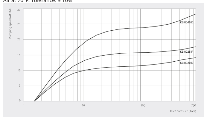
Pumping speed
