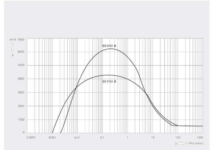
Pumping speed
