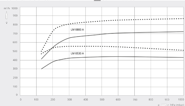
Pumping speed
