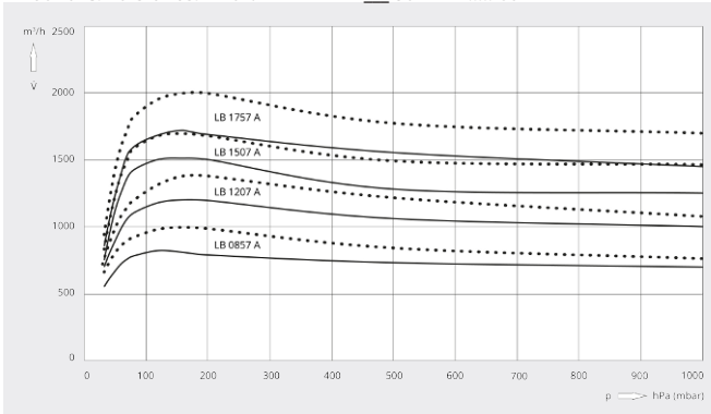
Pumping speed
