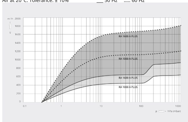
Pumping speed
