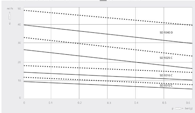
Volume flow
