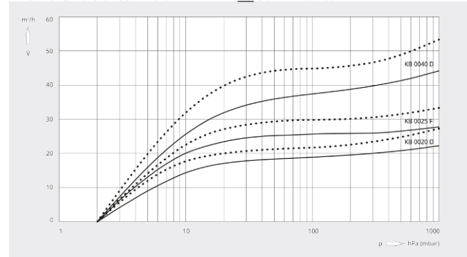
Pumping speed
