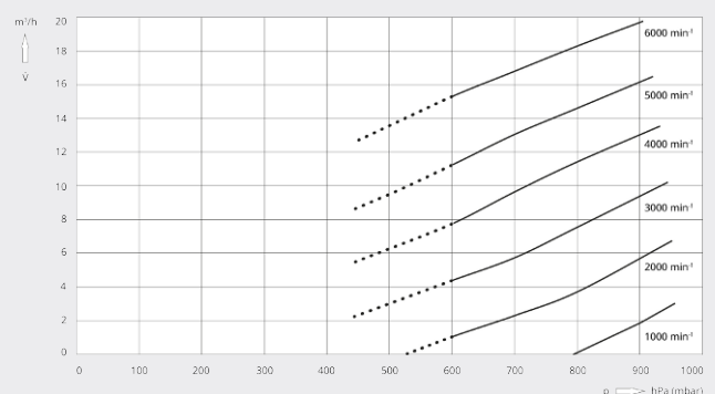
Pumping speed
