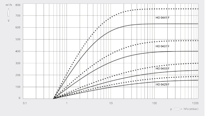
Pumping speed
