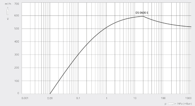
Pumping speed
