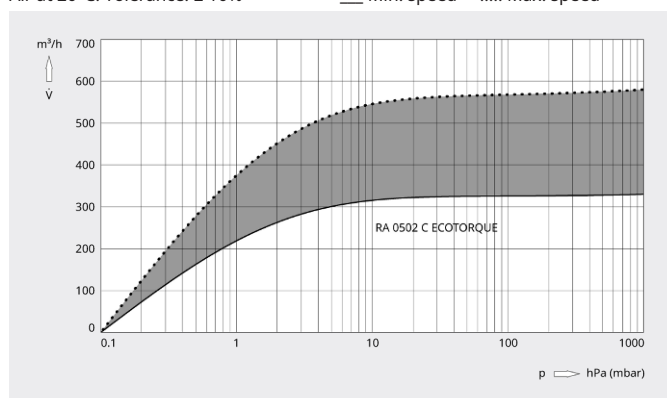
Pumping speed
