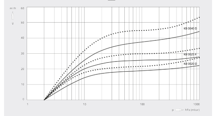
Pumping speed
