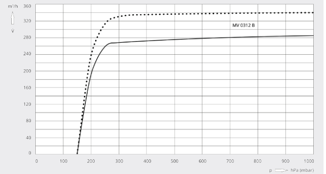
Pumping speed
