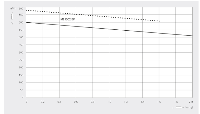
Volume flow Air at 20°C. Tolerance: \pm 10\%
