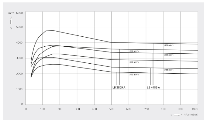
Pumping speed
