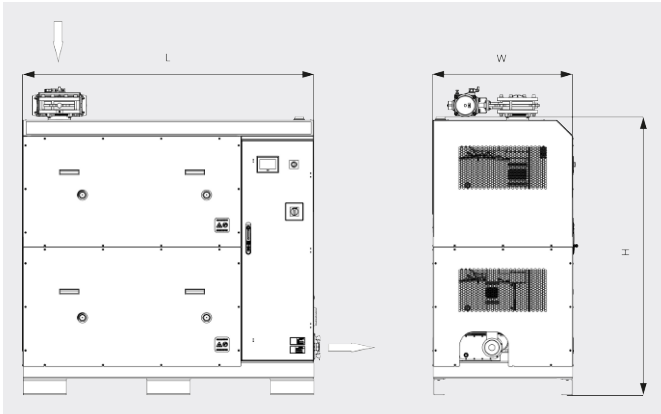
Dimensional drawing
