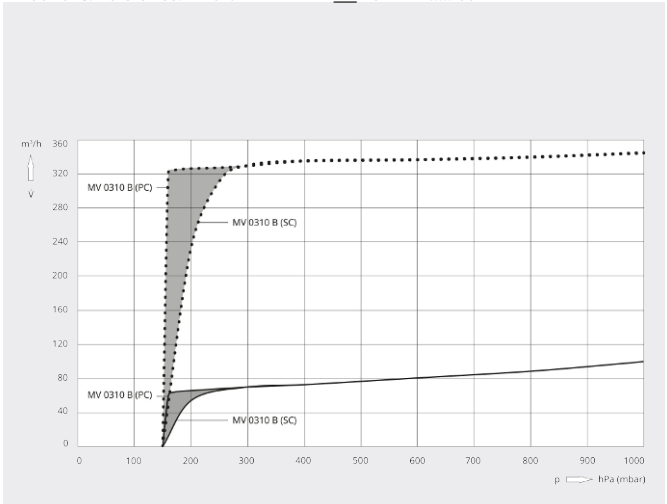
Pumping speed Air at 20°C. Tolerance: \pm 10\%
