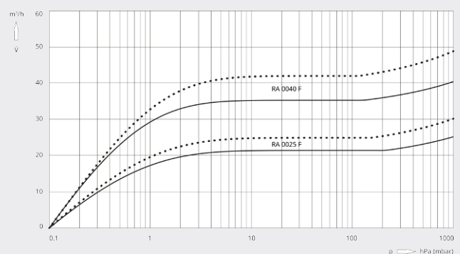
Pumping speed
