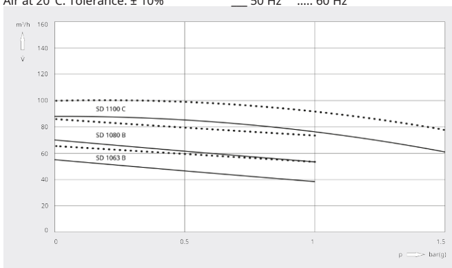
Volume flow
