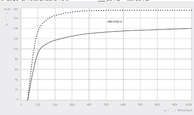
Pumping speed
