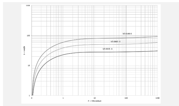
Pumping speed
