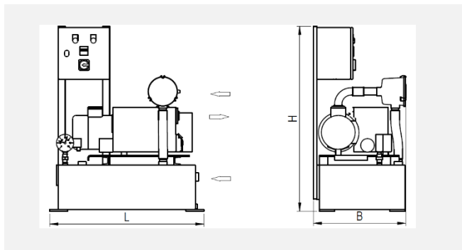
Dimensional drawing
