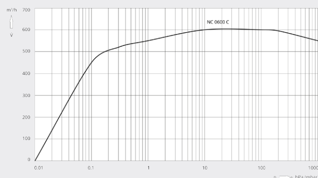
Pumping speed Air at 20°C. Tolerance: \pm 10\%
