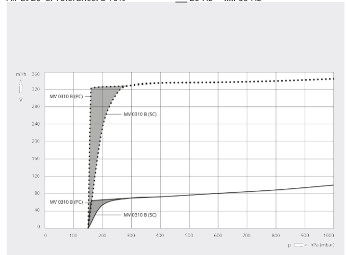
Pumping speed
