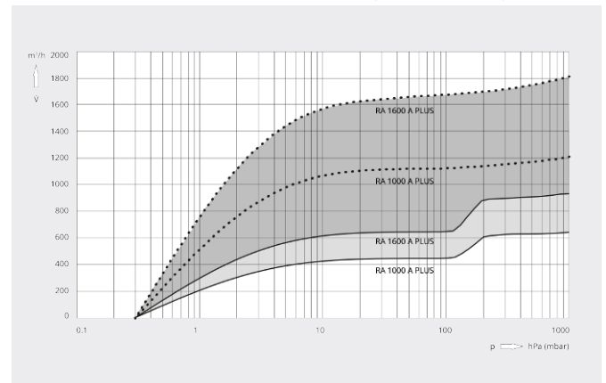
Pumping speed
