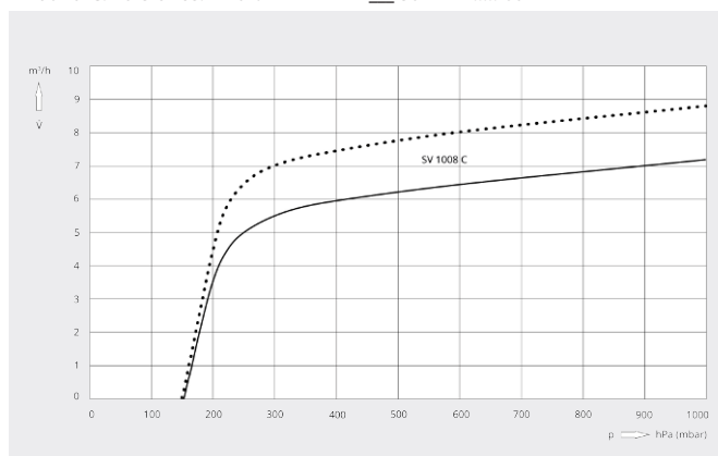
Pumping speed
