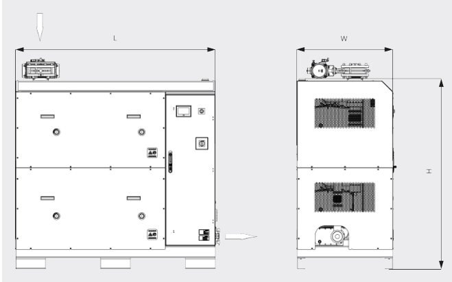
Dimensional drawing
