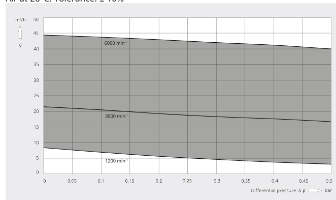
Volume flow (at inlet) Air at 20°C. Tolerance: \pm 10\%
