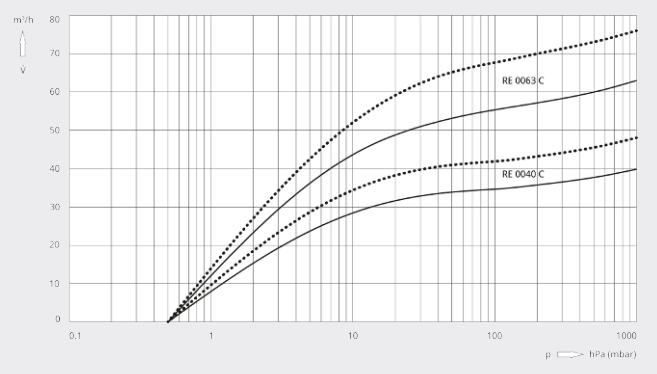
Pumping speed
