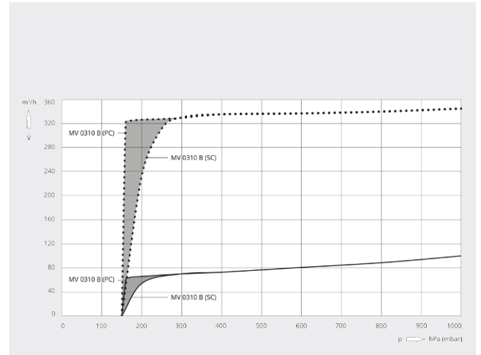
Pumping speed
