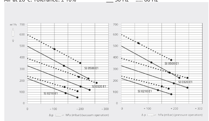
Pumping speed / Volume flow Air at 20°C. Tolerance: ± 10%
