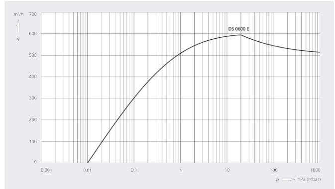
Pumping speed
