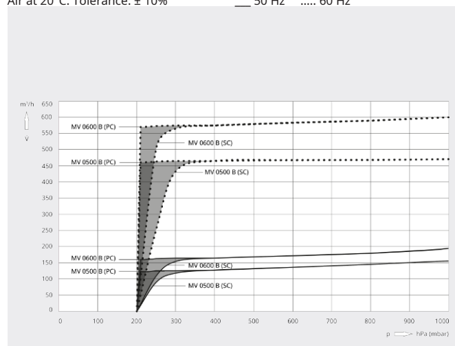
Pumping speed
