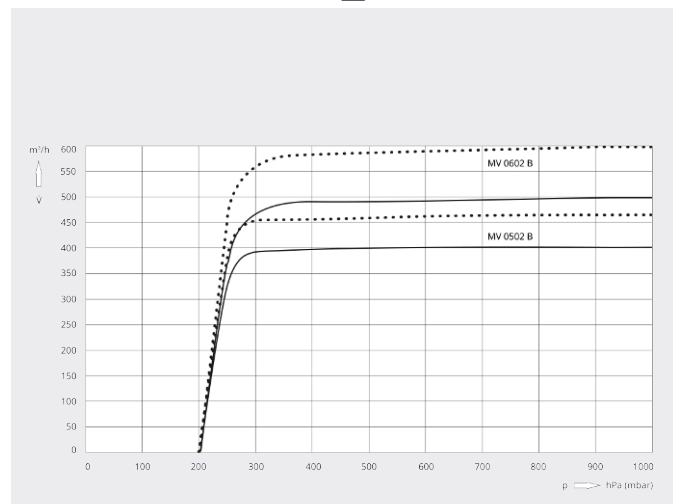
Pumping speed
