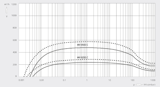
Pumping speed
