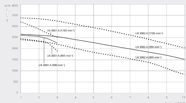
Pumping speed
