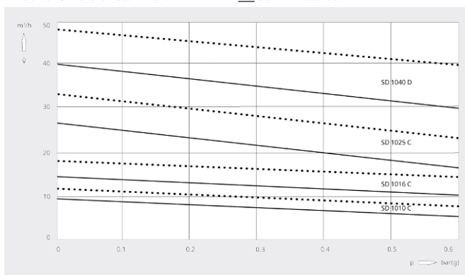
Volume flow
