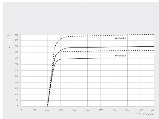
Pumping speed
