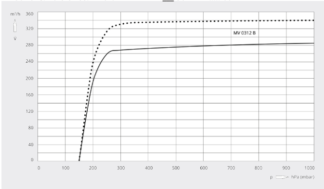
Pumping speed Air at 20°C. Tolerance: \pm 10\% — 50 Hz ..... 60 Hz
