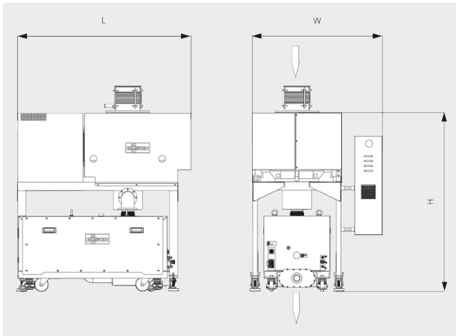
Plano dimensional
