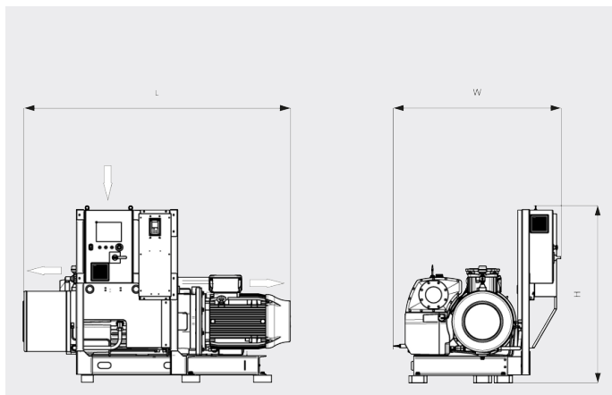
Dimensional drawing
