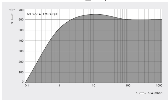
Pumping speed
