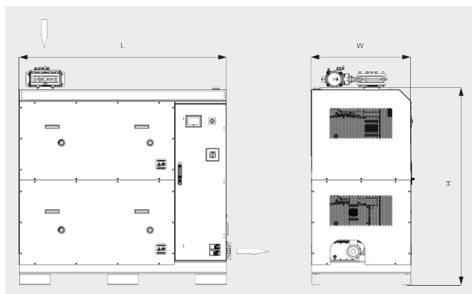
Dimensional drawing
