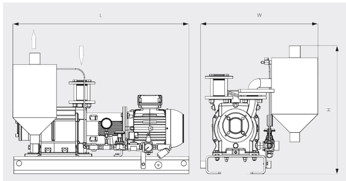
Dimensional drawing
