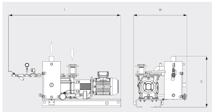
Dimensional drawing (Safe Area)
