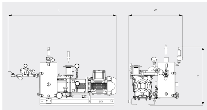
Dimensional drawing (ATEX)
